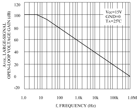
Figure 2. Open-Loop Frequency
